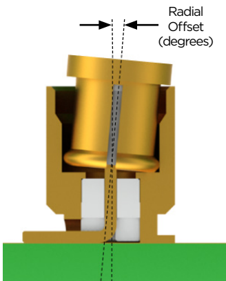
Figure 2: Radial Misalignment Measurement
